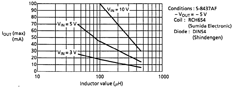
Figure 5 Inductor value – maximum output current *
