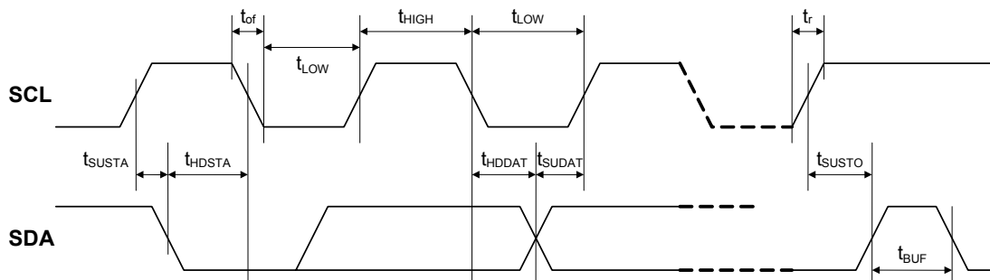
Figure 2. I 2 C Timing Parameters
