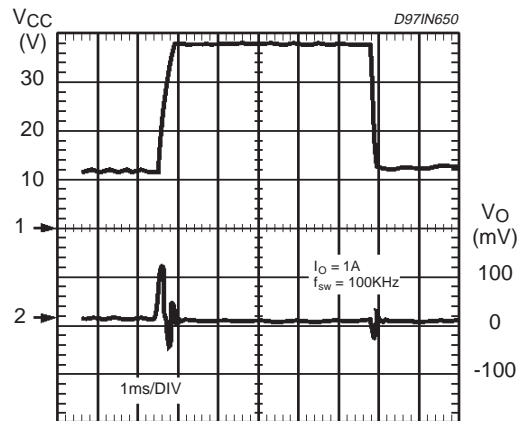
Figure 27: Line Transient
