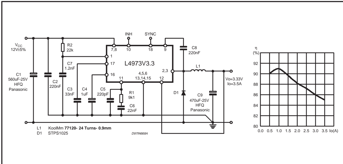
Figure 34: Synchronization Example
