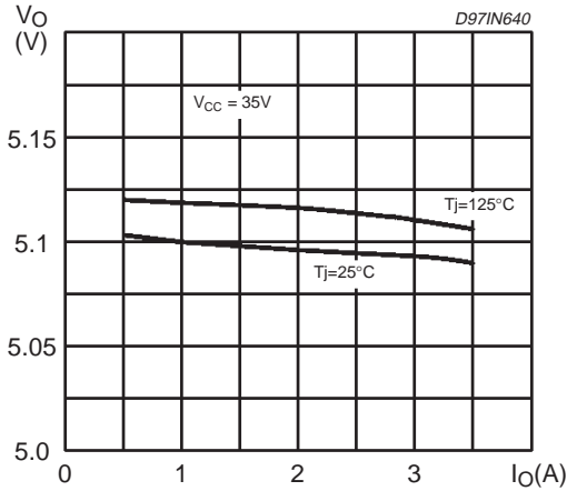
Figure 12: Load Regulation (see fig. 1d)
