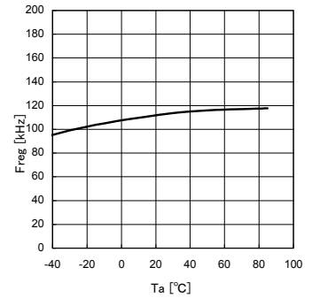
Fig.18 Switching
