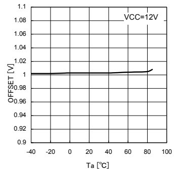
Fig.24 INV Pin Threshold voltage- Temperature
