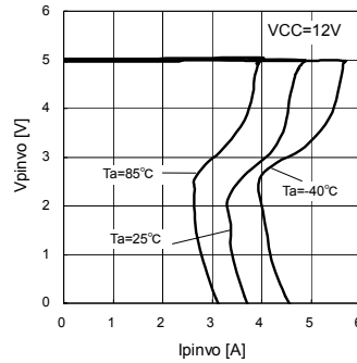
Fig.17 Over Current Protection
