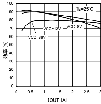
Fig.16 Efficiency - Load Current
