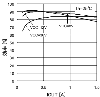
Fig.4 Efficiency-Load Current
