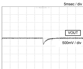
Fig.13 Load Response
