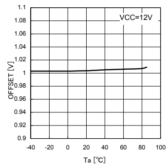
Fig.12 INV Pin Threshold voltage-Temperature
