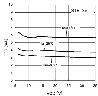
Fig.9 Circuit current-Supply voltage Iout=No Load
