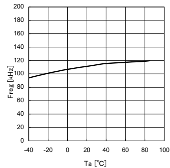
Fig.6 Switching Frequency-Temperature
