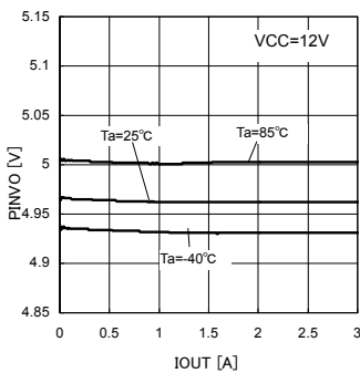
Fig.19 Output voltage - Load Current
