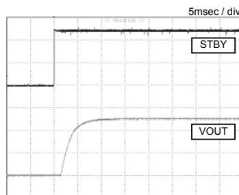
Fig.26 Start-up waveform
