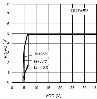
Fig.20 Output voltage-Supply voltage
