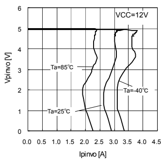
Fig.5 Over Current Protection
