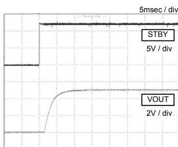
Fig.14 Start-up waveform
