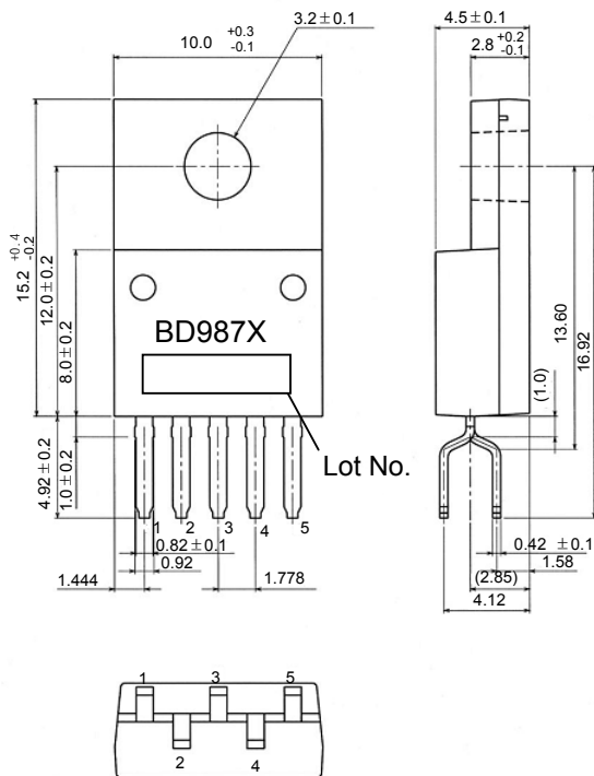
TO220CP-V5 (Unit : mm)
