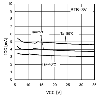
Fig.21 Circuit current-Supply voltage Iout= No Load
