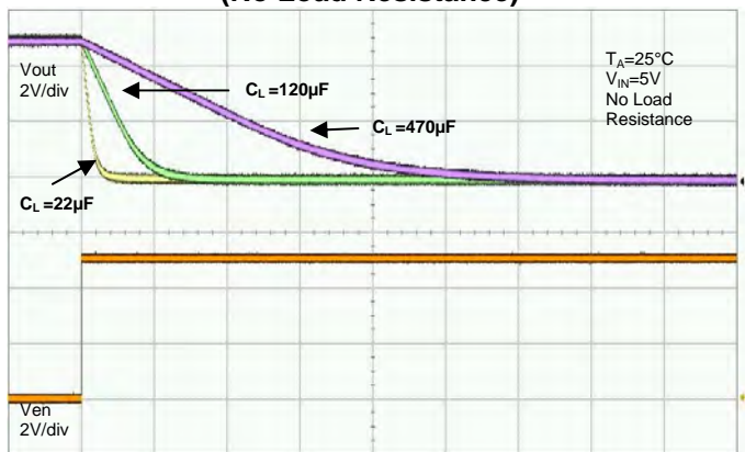
Discharge Time (No Load Resistance)
