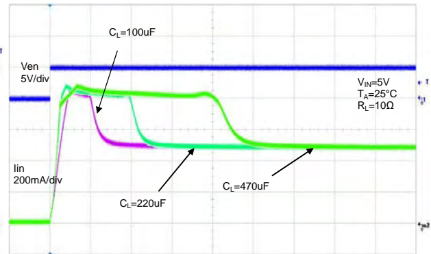
Inrush Current
