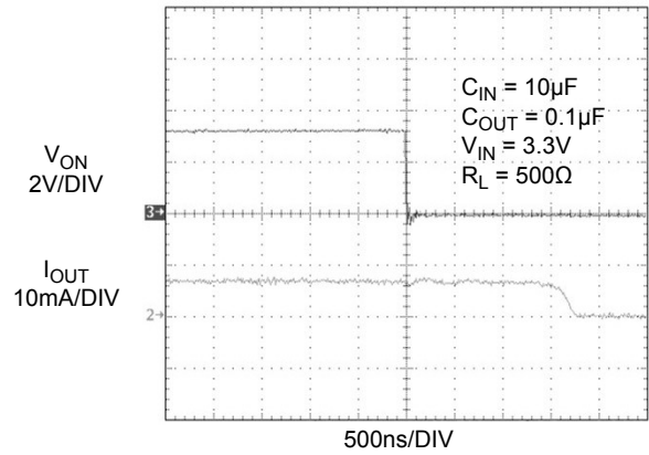
Figure 16. T_{DF} Response
