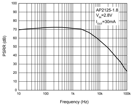
Figure 34. PSRR
