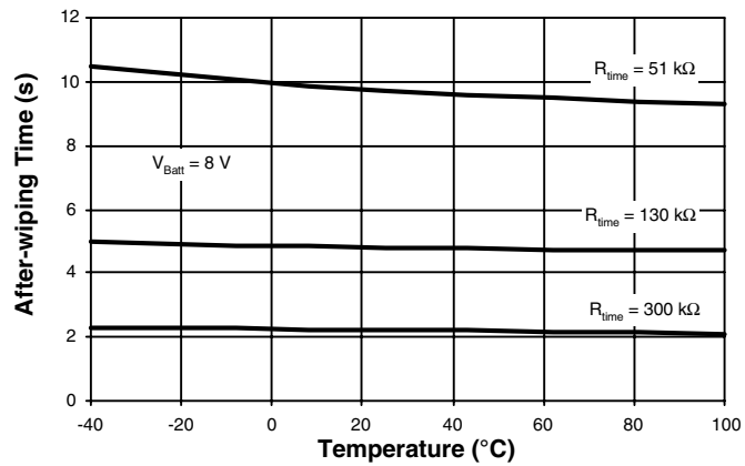
Figure 8-2. After-wiping Time = f(T) ; C_t = 22 \mu\text{F} ; V_{\text{Batt}} = 8 \text{ V}
