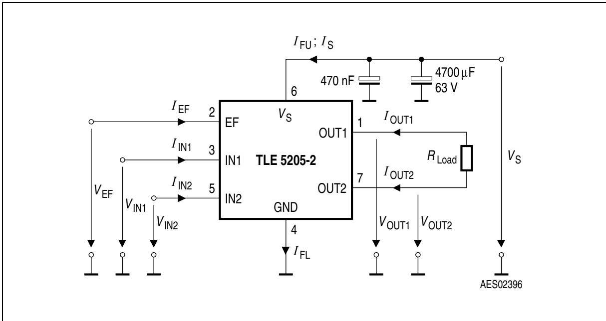
Figure 4 Test Circuit
