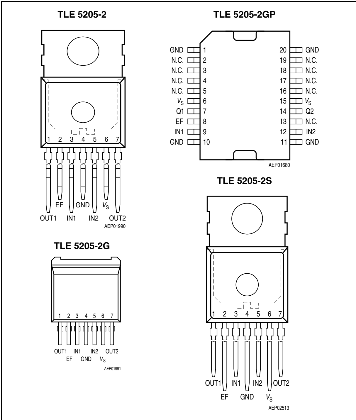
Figure 1 Pin Assignments
