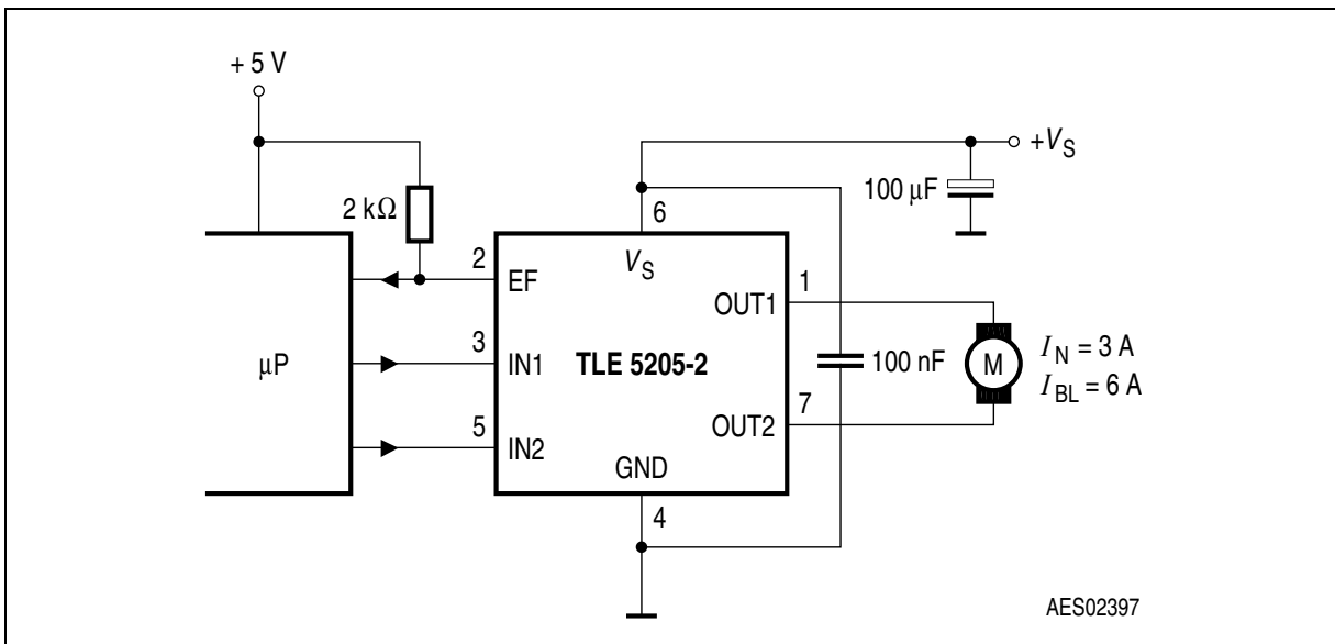
Figure 6 Application Circuit
