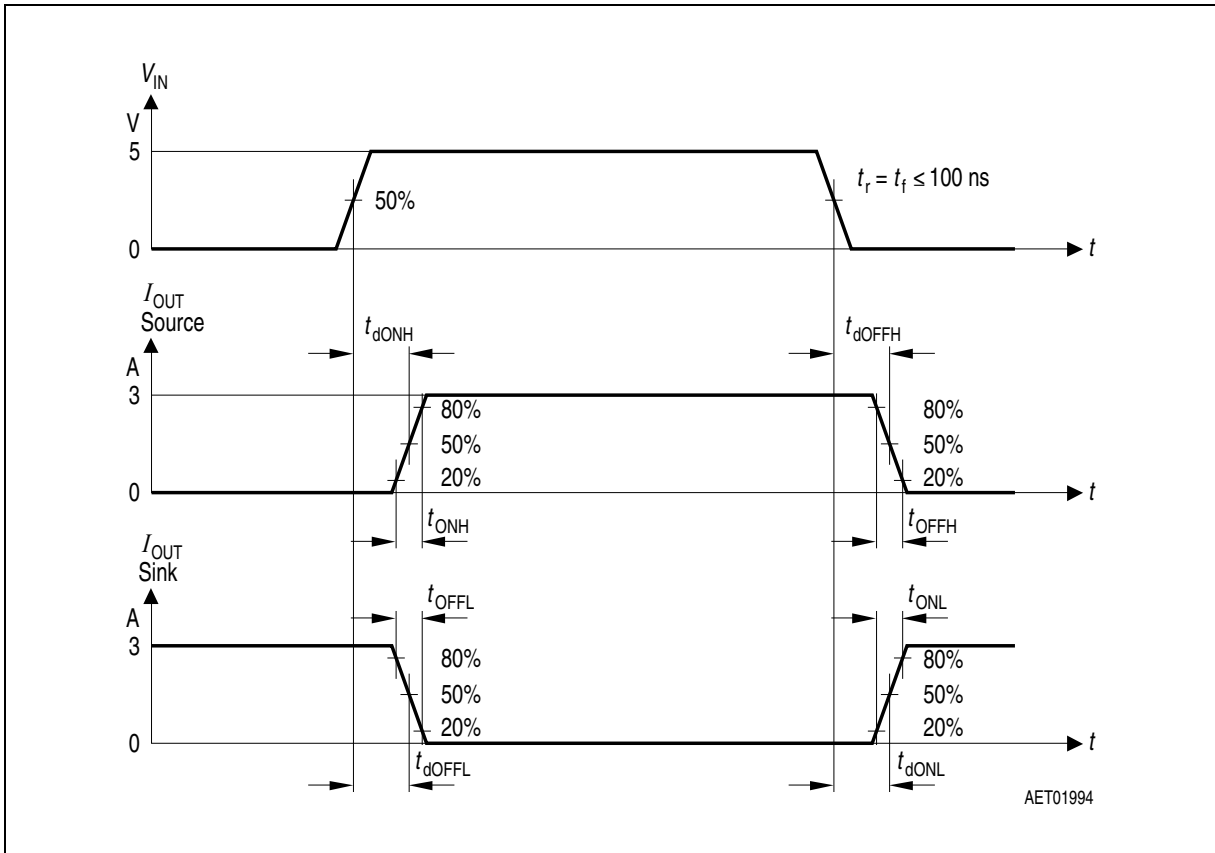
Figure 5 Switching Time Definitions
