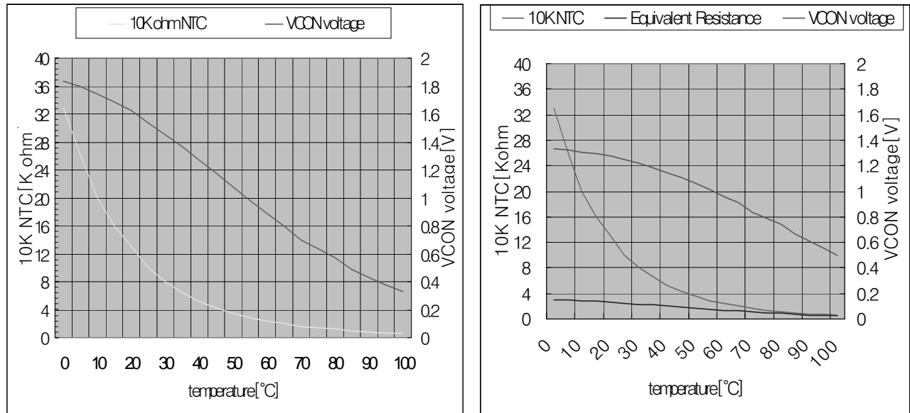
Figure 4. Sensed temperature and speed control voltage
