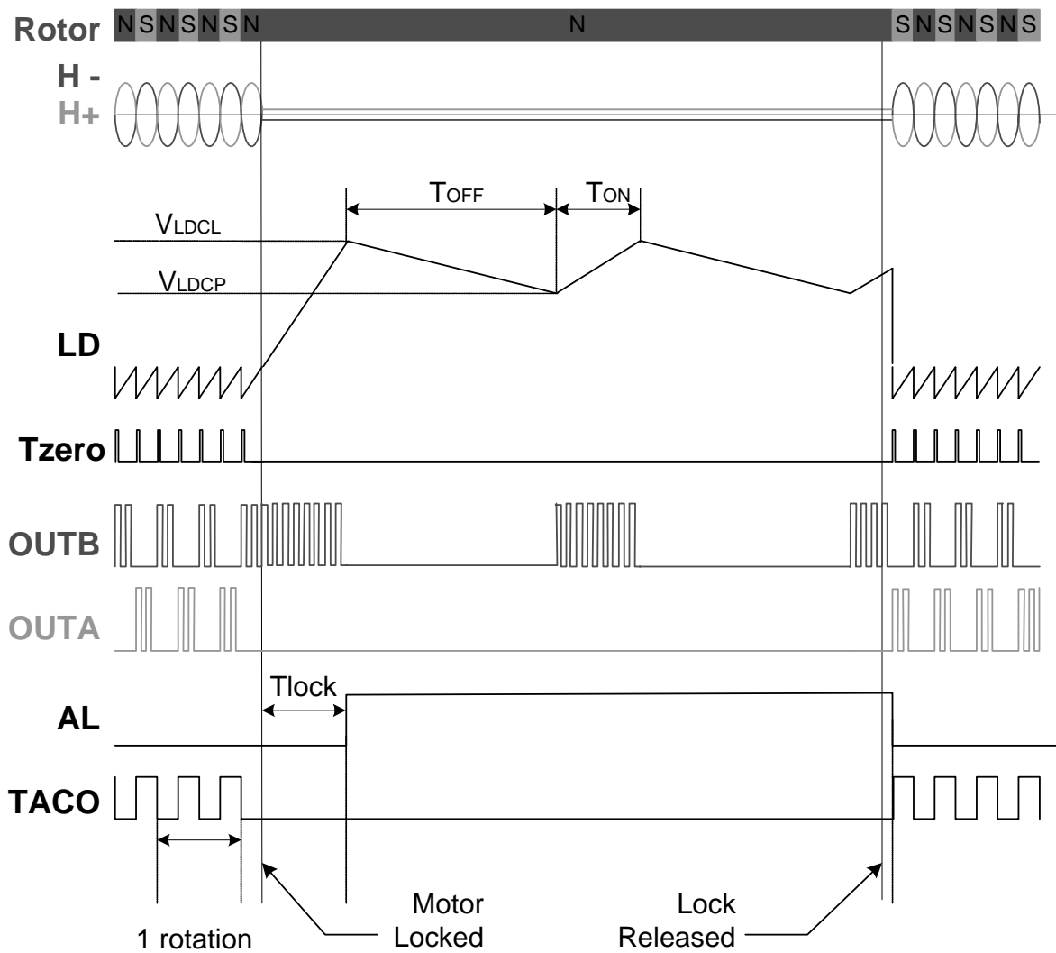
Figure 7. Overall Timing Chart
