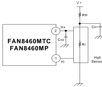
Figure 1. Hall Sensor Interface
