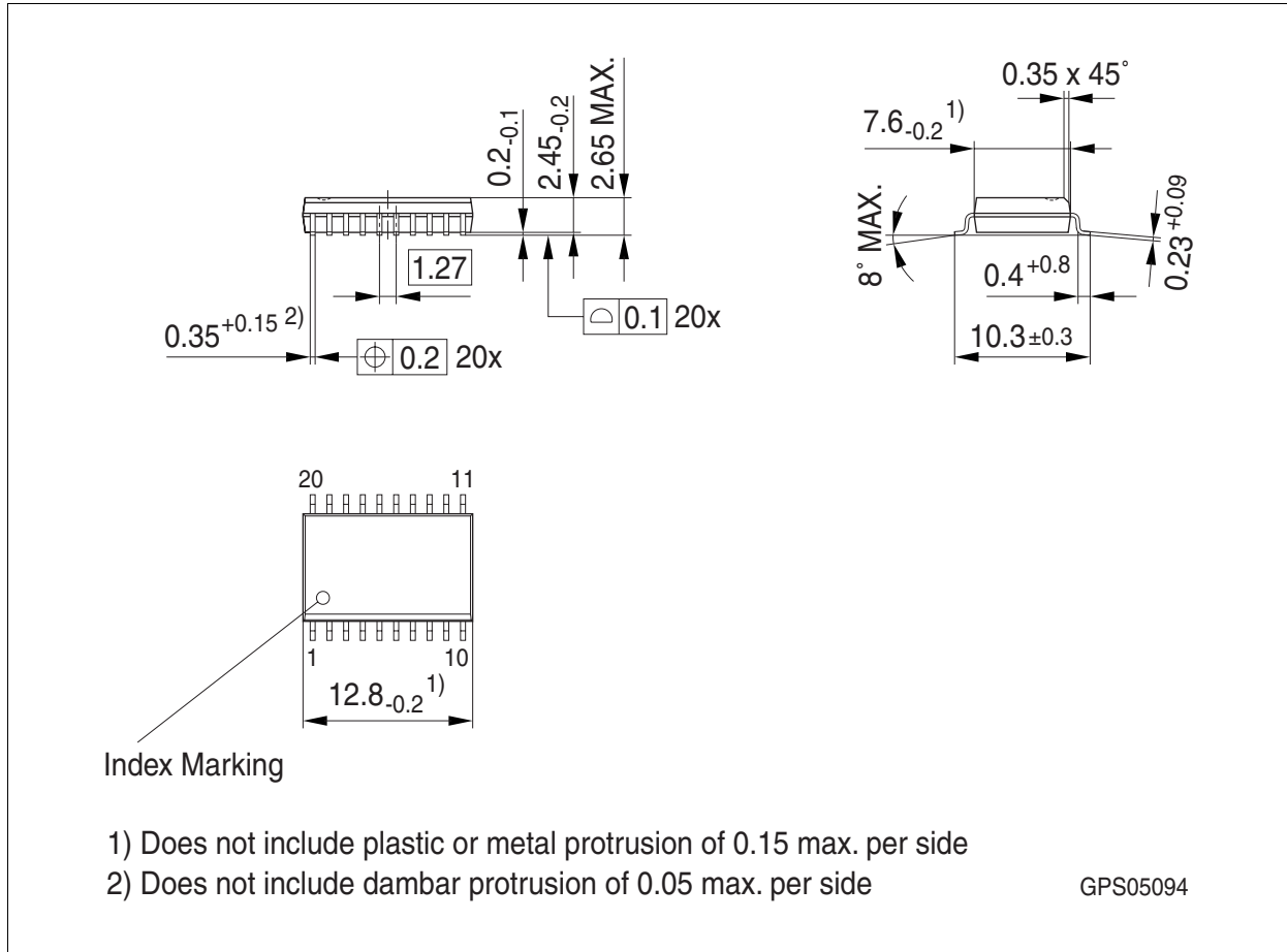
Figure 1 PG-DSO-20-32
