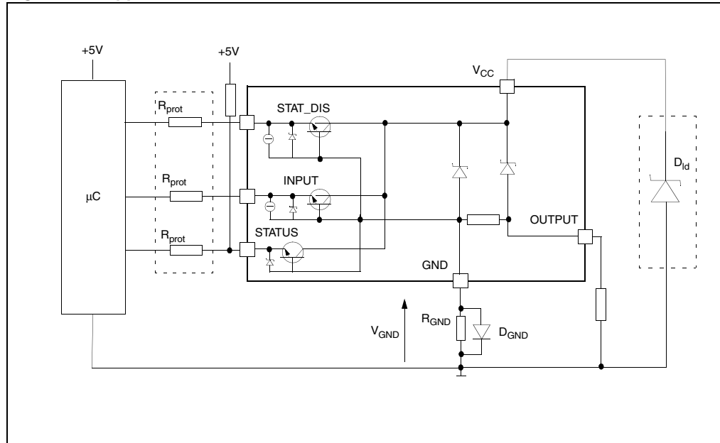
Figure 27. Application schematic
