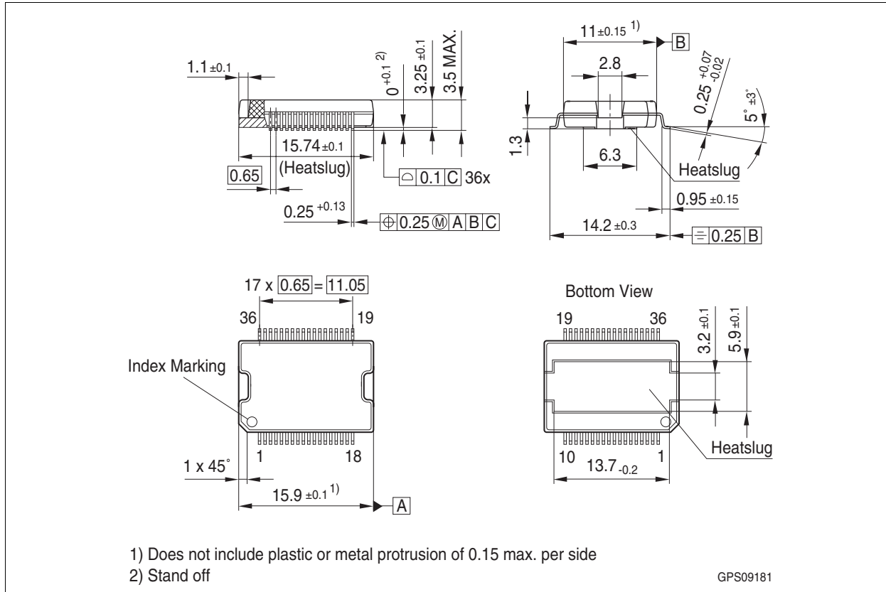
Figure 1 PG-DSO-36-26
