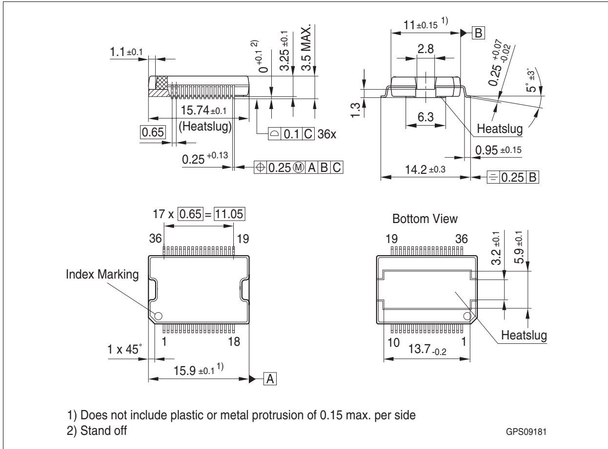
figure 6: PG-DSO-36
