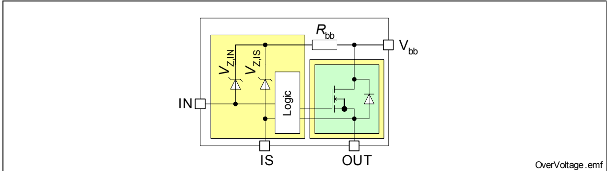
Figure 15 Over-Voltage Protection
