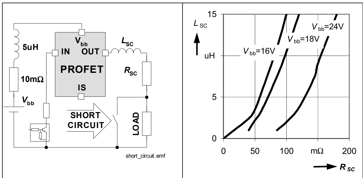
Figure 13 Short circuit
