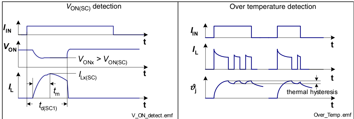
Figure 12 Overload Behavior
