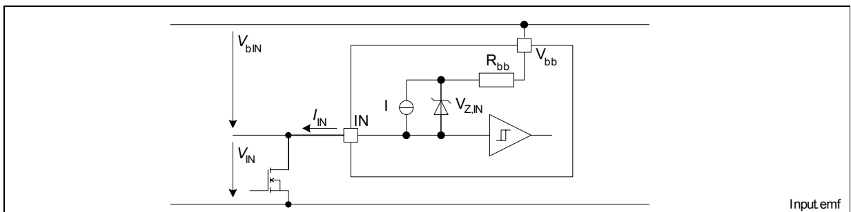
Figure 4 Input Circuit
