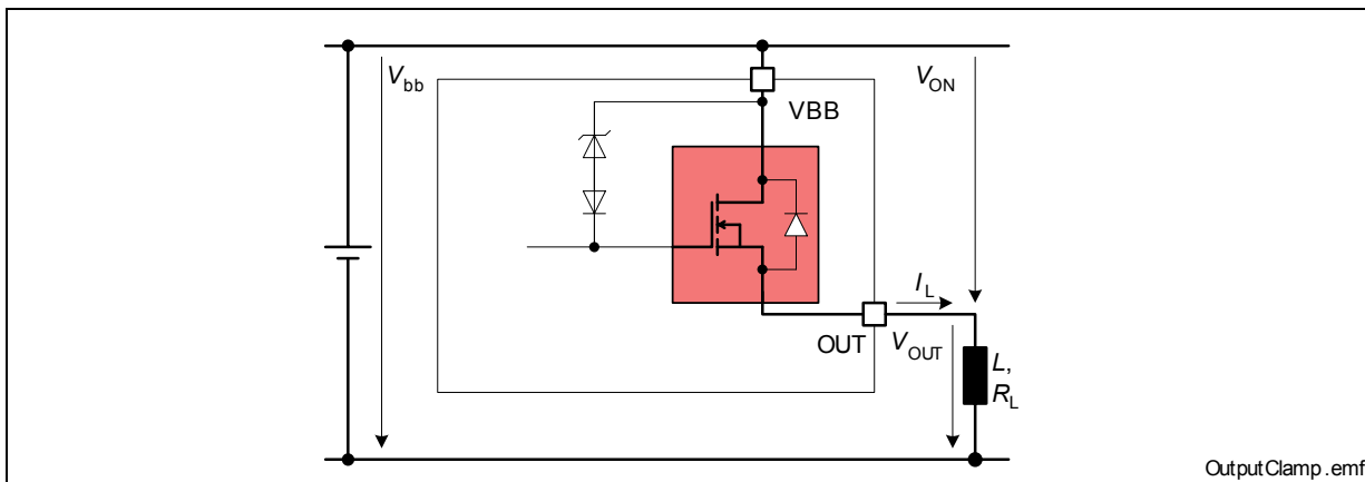
Figure 8 Output Clamp
