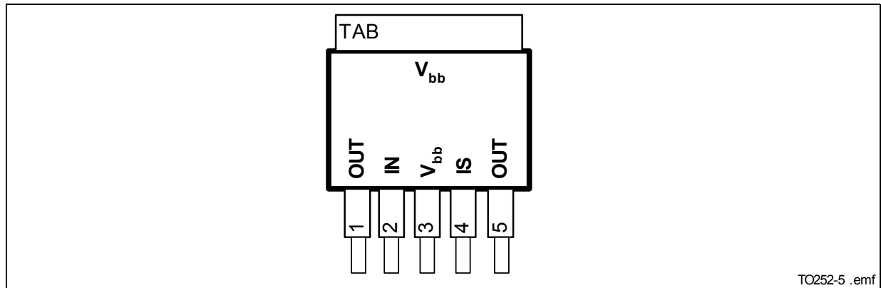
Figure 3 Pin Configuration PG-TO252-5-11
