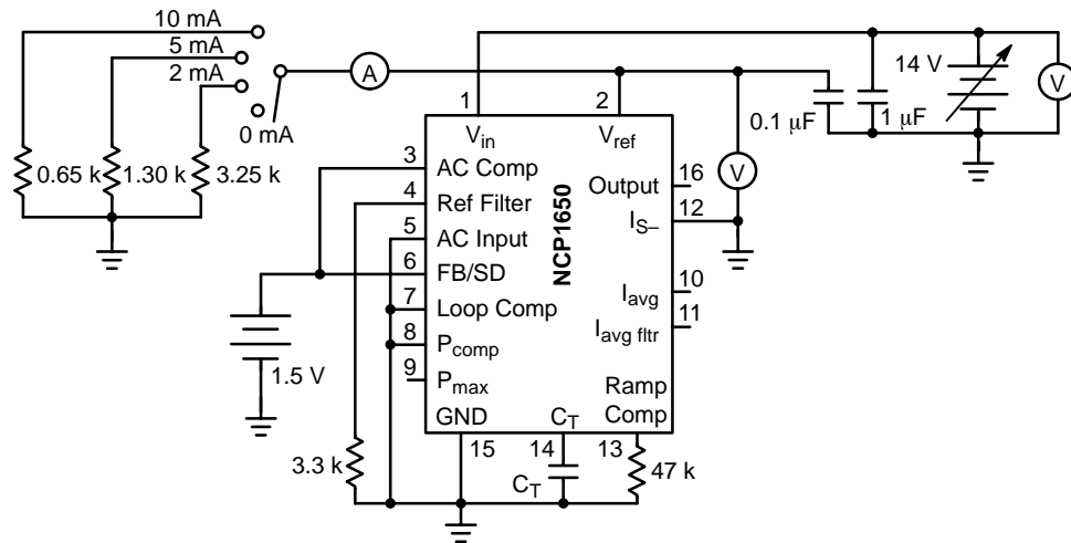
Figure 14. V_{ref} Line/Load Regulation in Operating Mode
