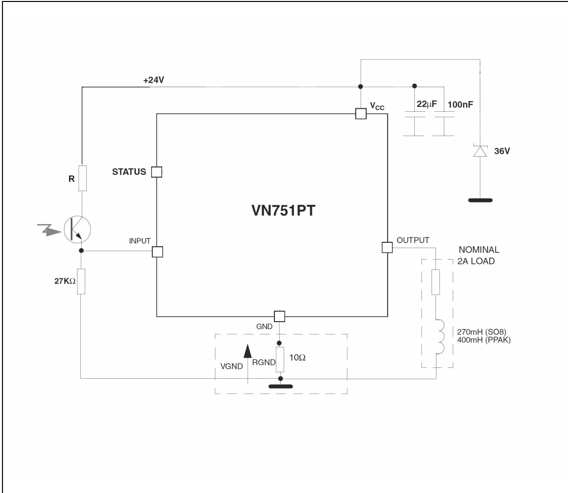
Figure 8. Application schematic
