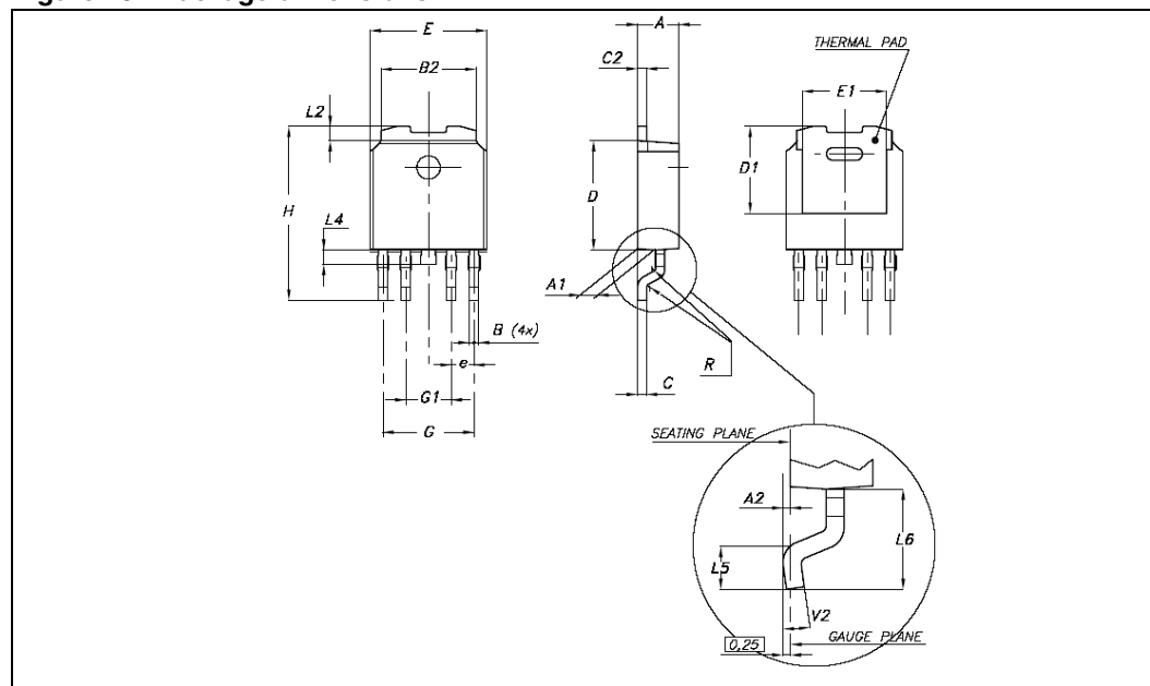
Figure 10. Package dimensions
