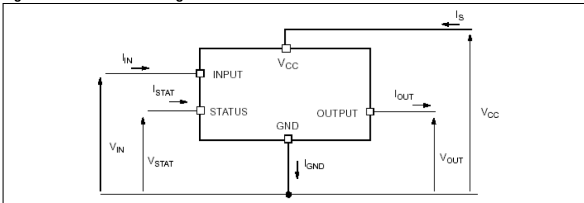
Figure 3. Current and voltage conventions
