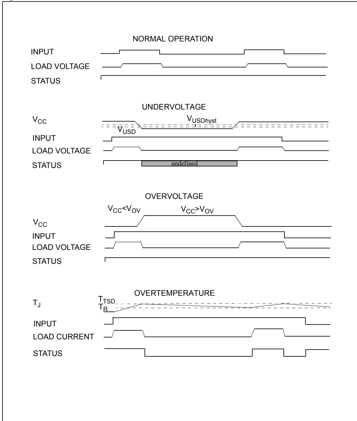
Figure 5. Waveforms
