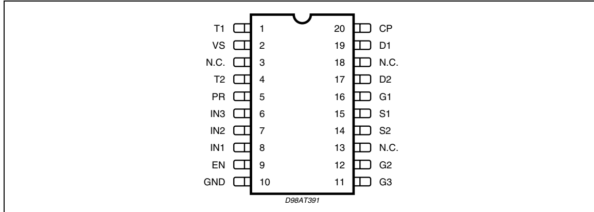
Figure 2. Pins connection (top view)
