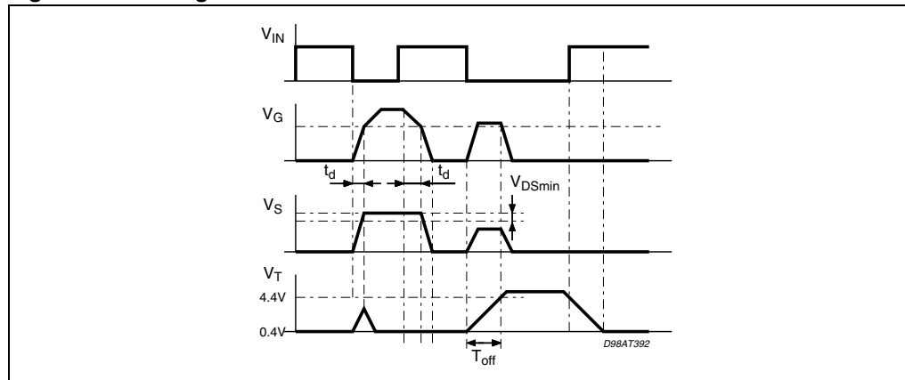
Figure 3. Timing characteristic
