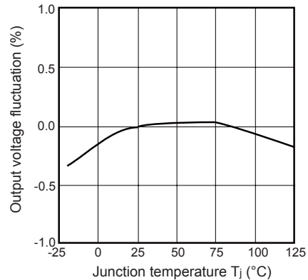
Fig.9 Output Voltage Fluctuation vs. Junction Temperature
