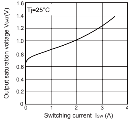
Fig.7 Output Saturation Voltage vs. Switching Current
