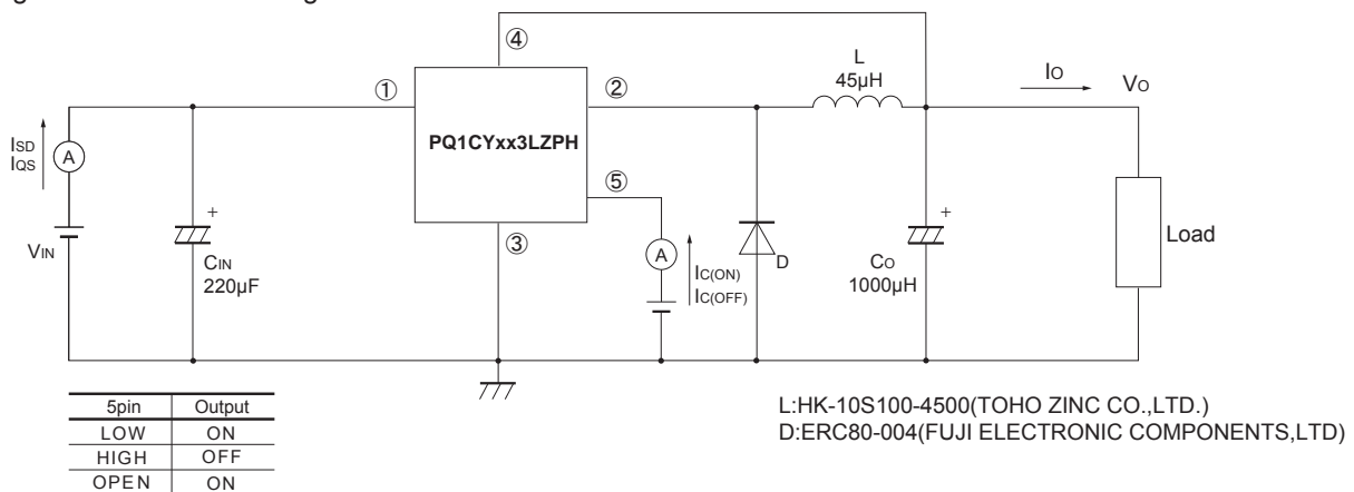
Fig.1 Standard measuring circuit
