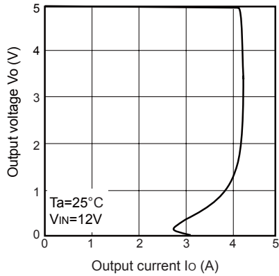
Fig.4 Overcurrent Protection Characteristics (PQ1CY503LZPH)
