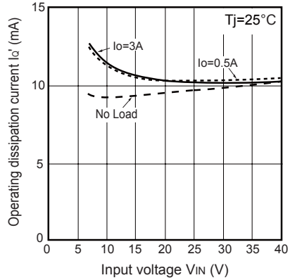
Fig.17 Operating Dissipation Current vs. Input Voltage (PQ1CY503LZPH)
