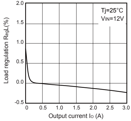
Fig.11 Load Regulation vs. Output Current(PQ1CY503LZPH)
