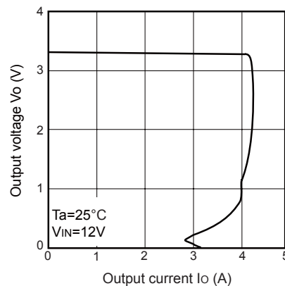
Fig.3 Overcurrent Protection Characteristics (PQ1CY333LZPH)
