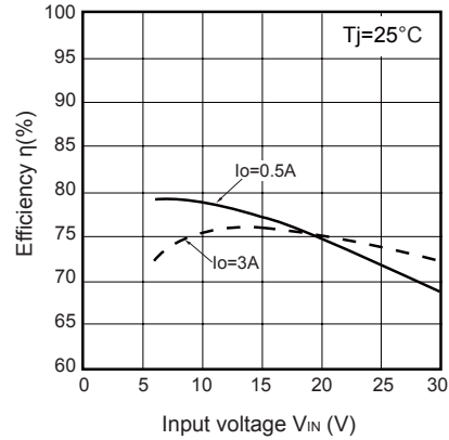
Fig.5 Efficiency vs. Input Voltage (PQ1CY333LH2PH)
