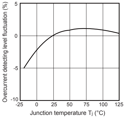
Fig.14 Overcurrent Detecting Level Fluctuation vs. Junction Temperature
