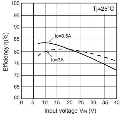
Fig.6 Efficiency vs. Input Voltage (PQ1CY503LH2PH)
