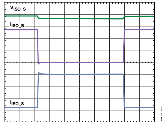
Figure 27. Load Transient. I_{ISO\_Sx} Load = 300 mA to 1500 mA to 300 mA, EN\_CHG = High , ILIM[3:0] = 0110 (Binary) = 500 mA
