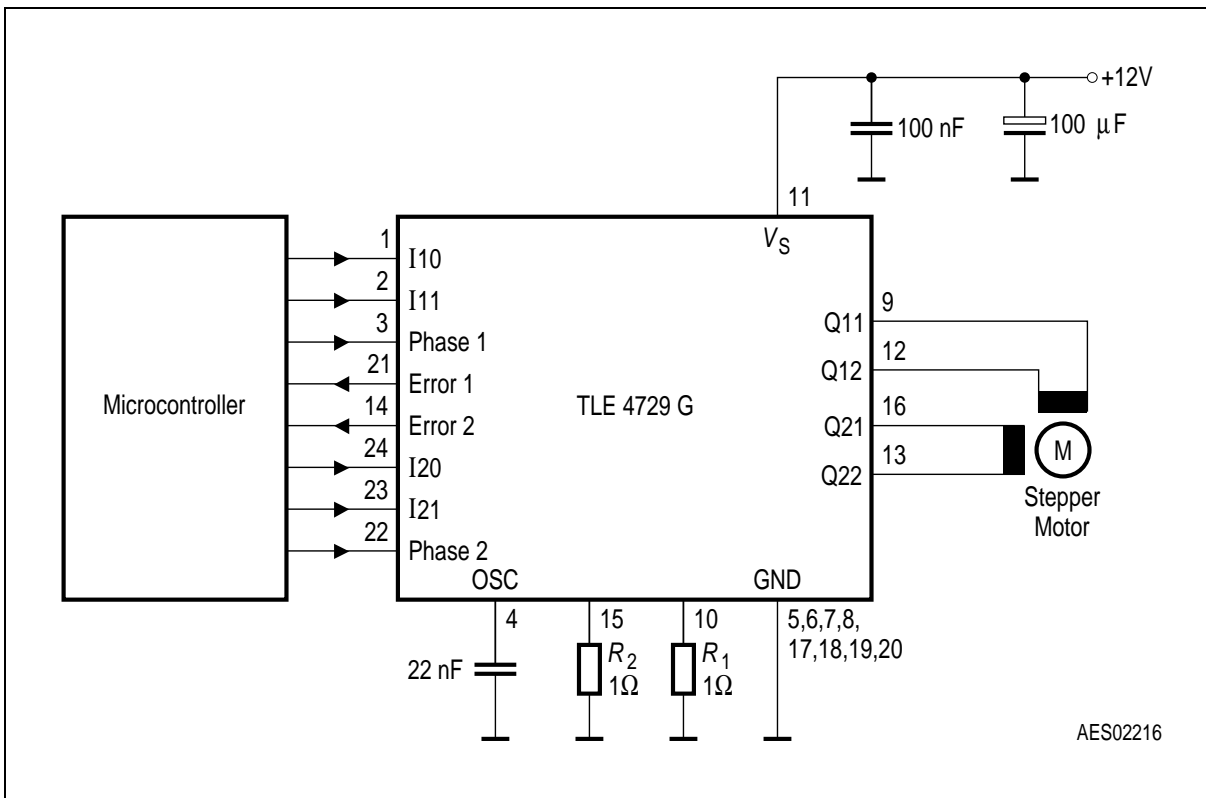
Figure 3 Application Circuit
