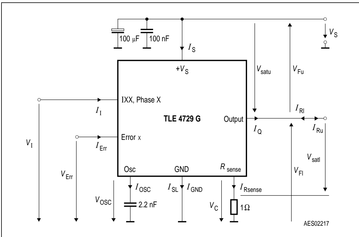
Figure 4 Test Circuit
