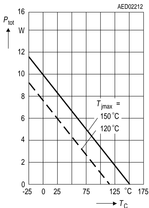
Permissible Power Dissipation P_{tot} vs. Case Temp. T_C (measured at pin 5)
