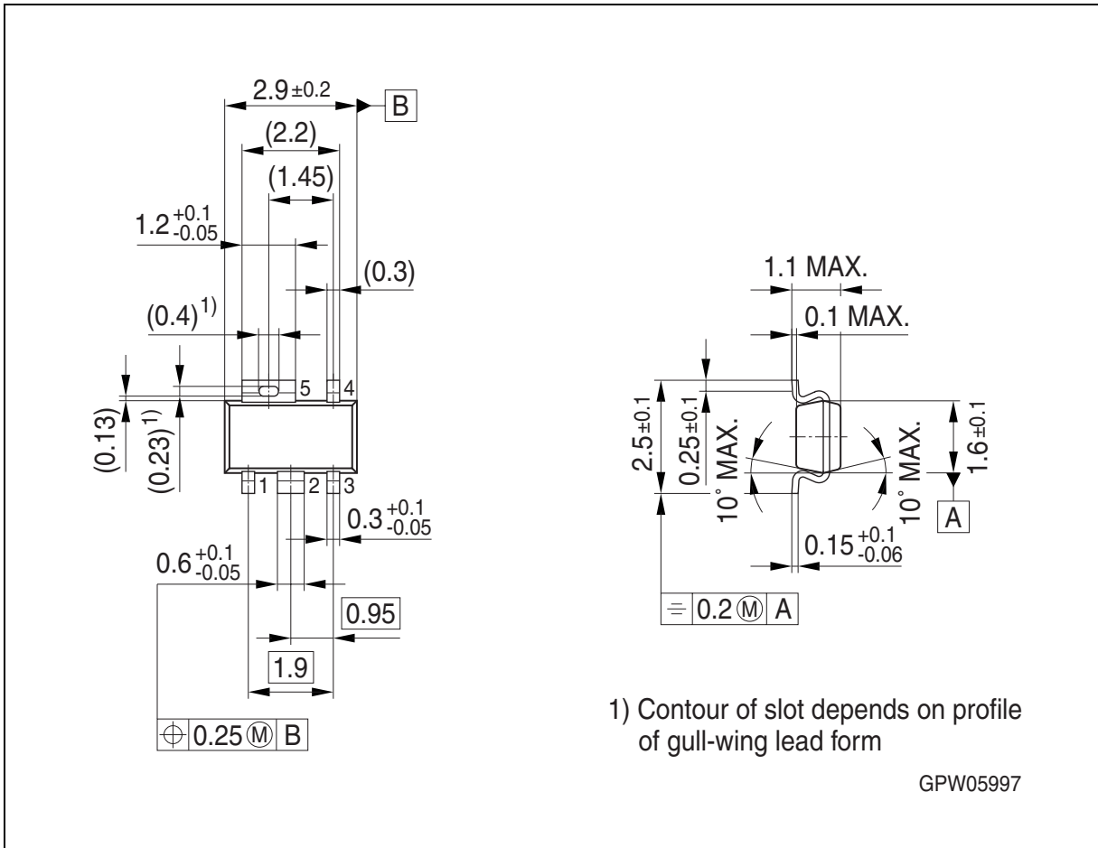
Figure 4 Outline PG-SCT595-5
