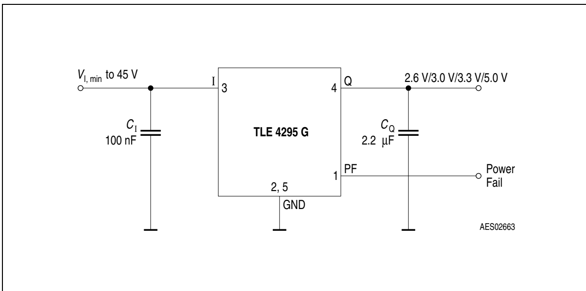
Figure 3 Application Circuit
