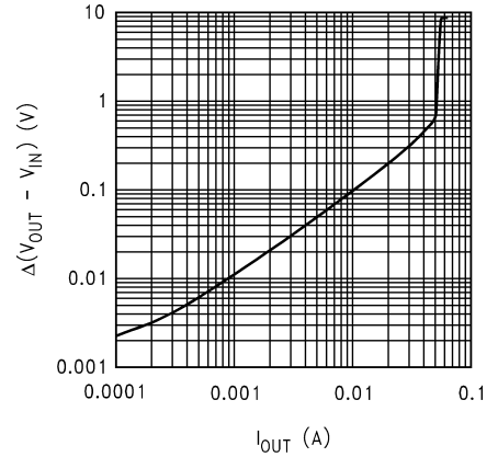
Output Voltage vs. Output Current (Vcom or Gamma, sinking)
