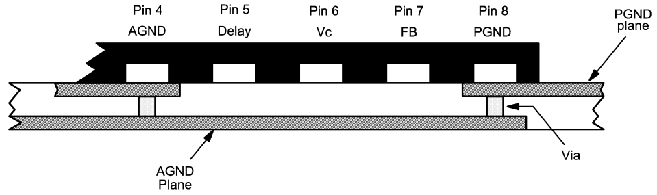
FIGURE 3. Multi-Layer Layout
