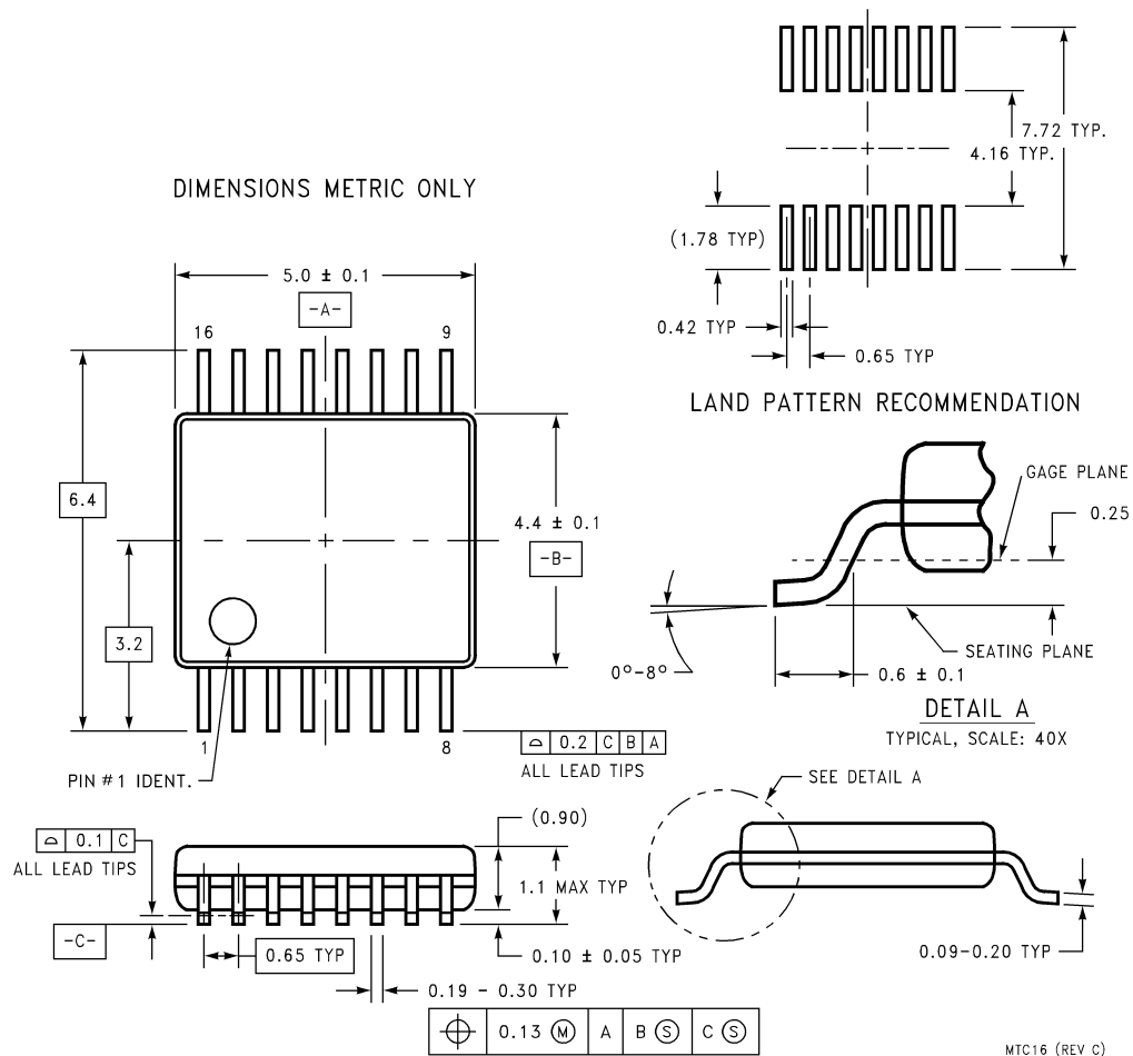
TSSOP-16 Pin Package (MTC) For Ordering, Refer to Ordering Information Table NS Package Number MTC16
