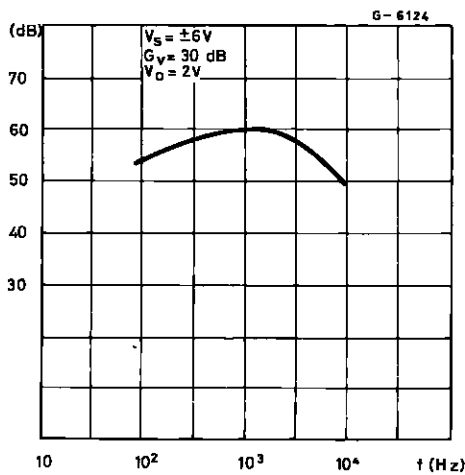
Figure 7 : Channel Separation versus Frequency
