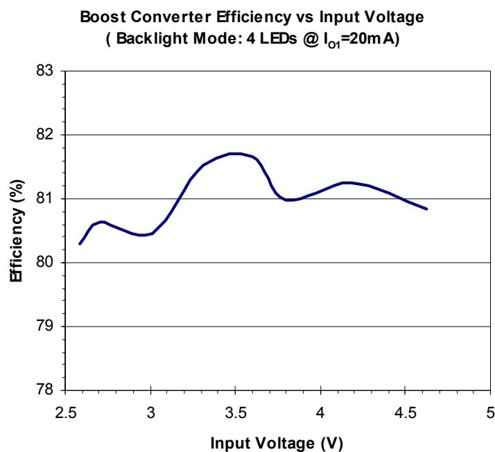
Figure 7b Efficiency Curve for Backlight LEDs Driver Application
