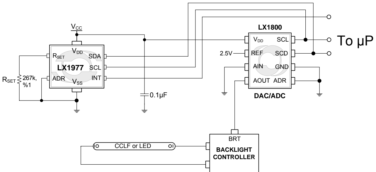
Figure 6 – Typical Application 2
