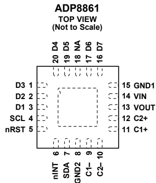
Figure 3. Pin Configuration
