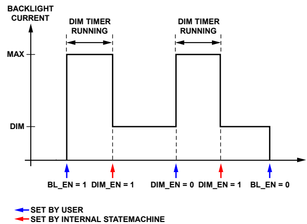
Figure 32. Dim Timer
