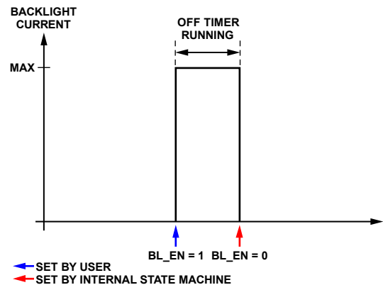
Figure 33. Off Timer
