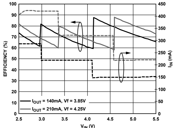
Figure 19. Typical Efficiency (High Vf Diode)
