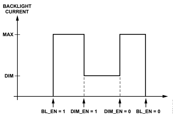
Figure 31. Backlight Turn On/Dim/Turn Off
