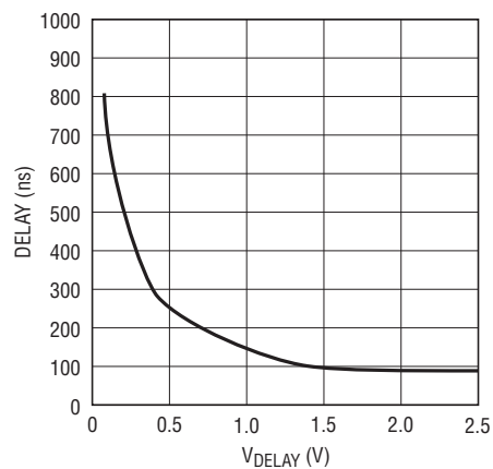
SGATE (Low) to BGATE (High) Delay vs V_{DELAY} ( R_{SET} = 80k )
