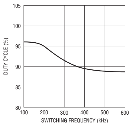
Switching Frequency vs Duty Cycle
