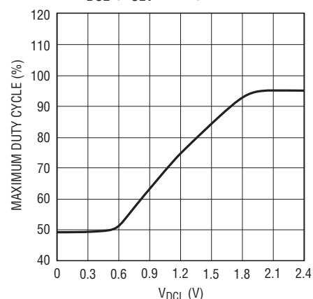
Maximum Duty Cycle Limit vs V_{DCL} ( R_{SET} = 80k )
