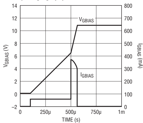
V_{GBIAS} vs I_{GBIAS} at Start-Up (Charging 2\mu\text{F} )
