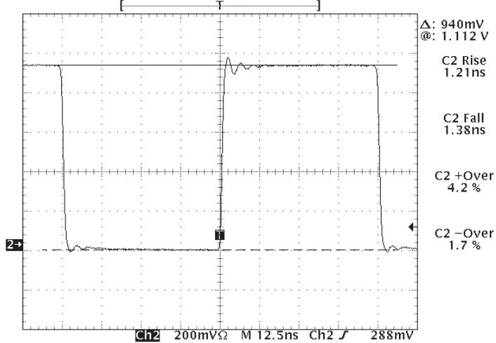
Figure 9-6. Output Pulse, Read: 50 mA, Write: 250 mA pk-pk
