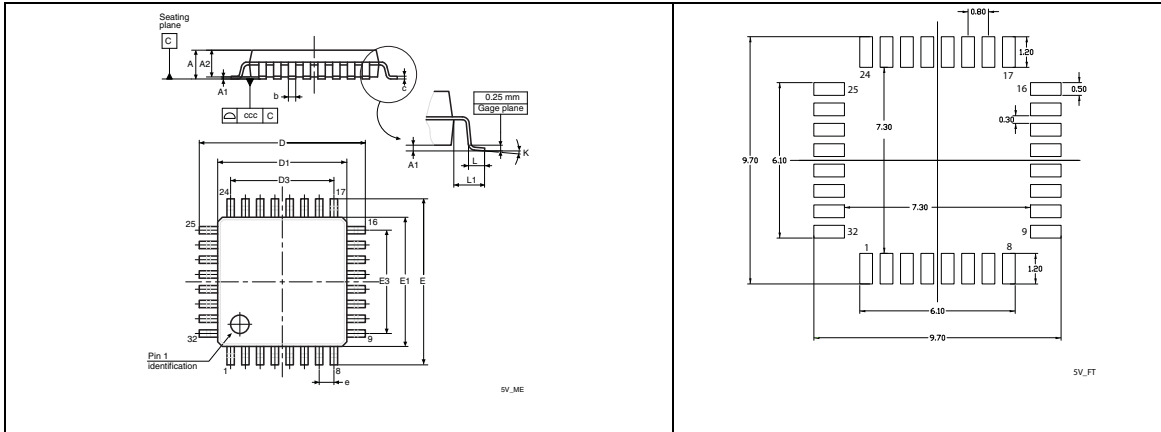
Figure 39. LQFP32 - 32-pin low profile quad flat package outline (7 x 7) (1)
