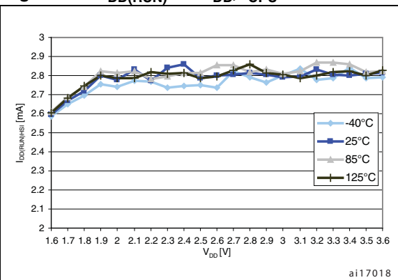
Figure 12. I_{DD(RUN)} vs. V_{DD} , f_{CPU} = 16\text{ MHz}
