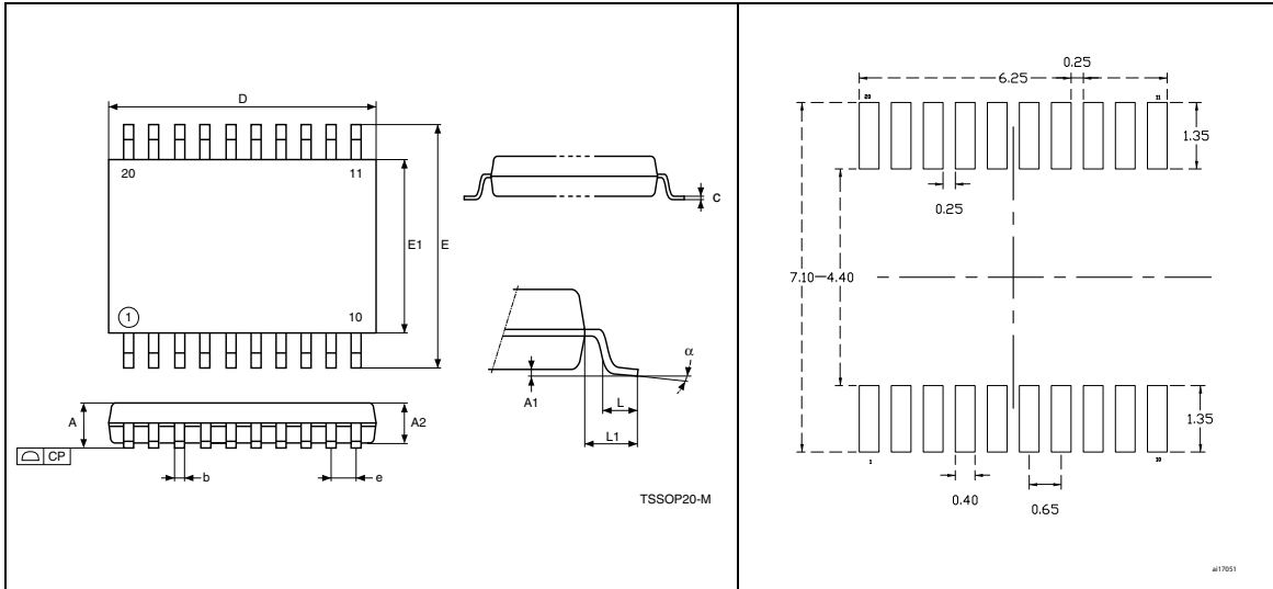
Figure 45. TSSOP20 - 20-lead thin shrink small package outline (1)
