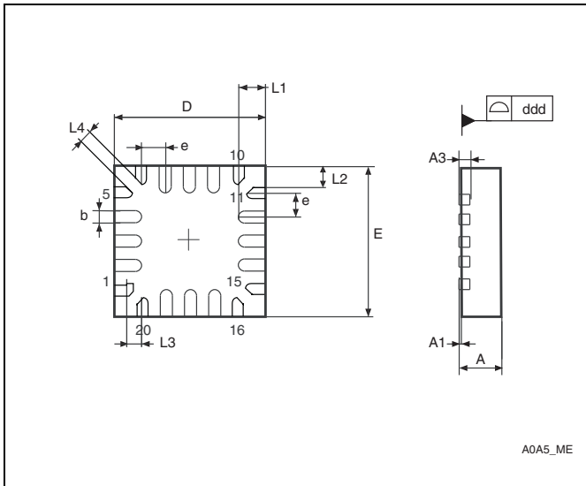
Figure 43. UFQFPN20 3 x 3 mm 0.6 mm package outline (1)
