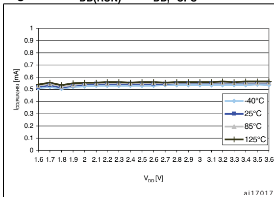
Figure 11. I_{DD(RUN)} vs. V_{DD} , f_{CPU} = 2\text{ MHz}
