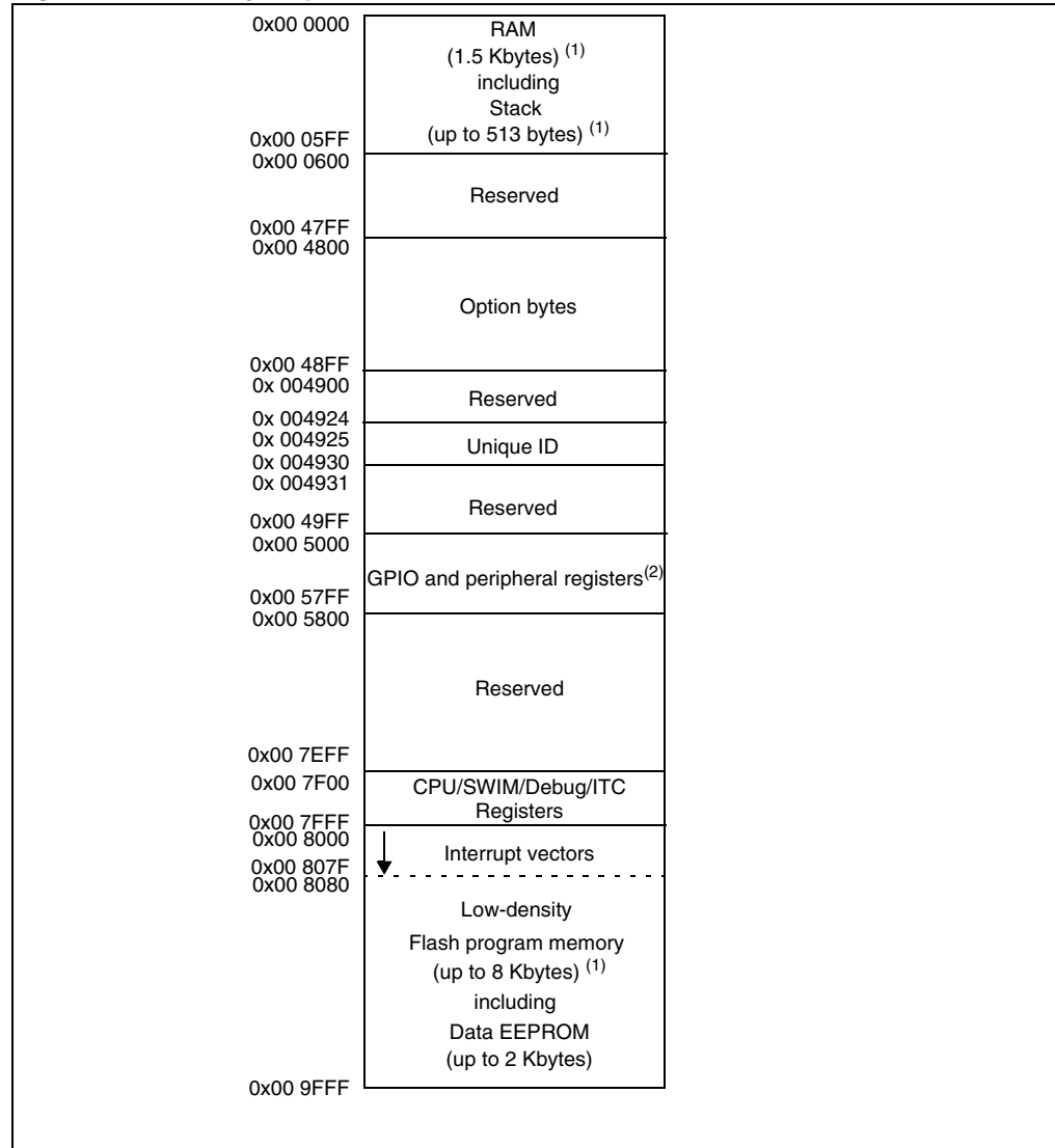
Figure 8. Memory map
