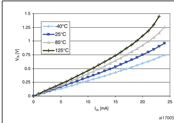
Figure 24. Typ. V_{OL} at V_{DD} = 3.0 V (standard ports)
