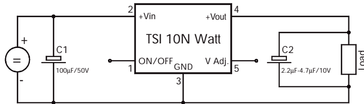
Normal Connection (Standard)
