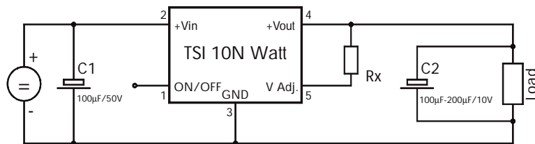
Output Voltage Adjustment Connection
