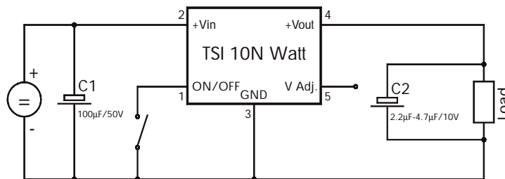
Remote ON/OFF Connection
