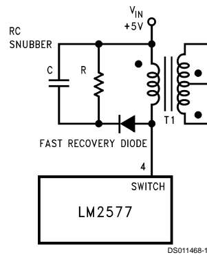
FIGURE 21. Snubber Circuit
