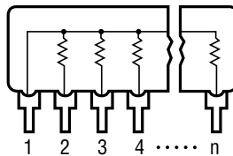
-1 Circuit Bussed Resistors
