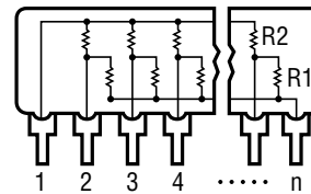
-5 Circuit Dual Terminator
