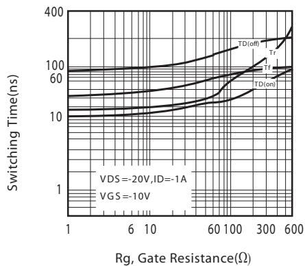
Figure 11. switching characteristics
