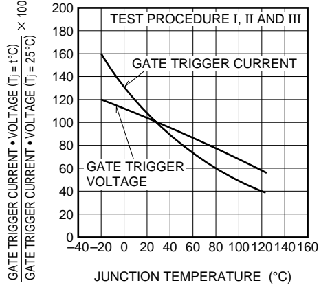
GATE TRIGGER CURRENT-VOLTAGE VS. JUNCTION TEMPERATURE
