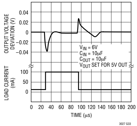
Transient Response C_{BYP} = 0.01\mu F
