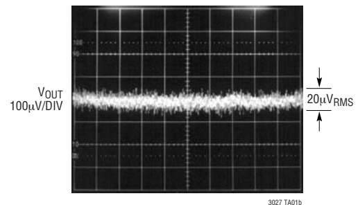
10Hz to 100kHz Output Noise
