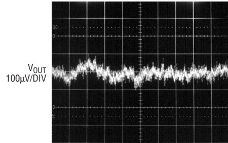
C_{OUT} = 10\mu F 1ms/DIV 3024 G44 I_L = 100mA V_{OUT} SET FOR 5V
