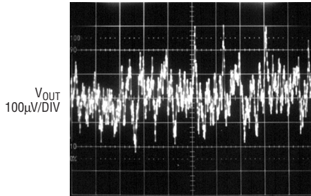
C_{OUT} = 10\mu F 1ms/DIV 3024 G43 I_L = 100mA V_{OUT} SET FOR 5V
