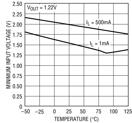
Output 1 Minimum Input Voltage
