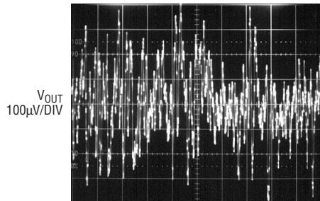
C_{OUT} = 10\mu F 1ms/DIV 3024 G42 I_L = 100mA V_{OUT} SET FOR 5V
