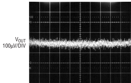
C_{OUT} = 10\mu F 1ms/DIV 3024 G45 I_L = 100mA V_{OUT} SET FOR 5V
