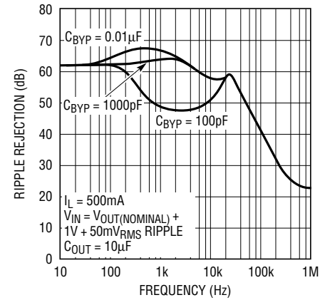
Output 1 Input Ripple Rejection
