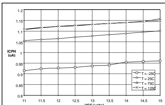
Figure 40: ICPH versus VCC and temperature
