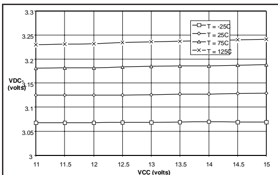
Figure 37: VDC- threshold versus VCC and temperature
