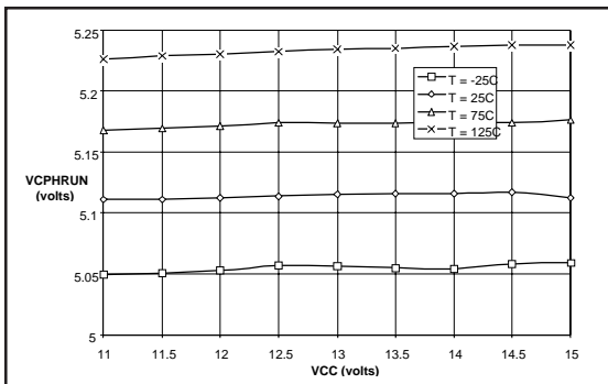
Figure 39: VCPHRUN threshold versus VCC and temperature
