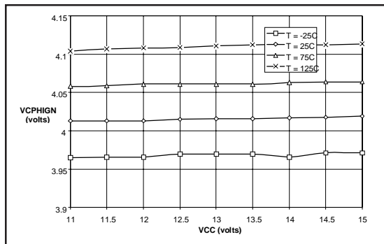
Figure 38: VCPHIGN threshold versus VCC and temperature
