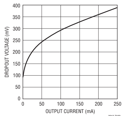
Dropout Voltage
