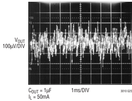
LT3010-5 10Hz to 100kHz Output Noise
