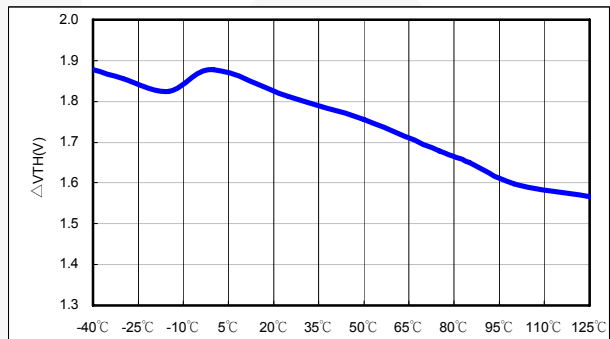
Figure 10. \Delta V_{TH} vs. Temperature
