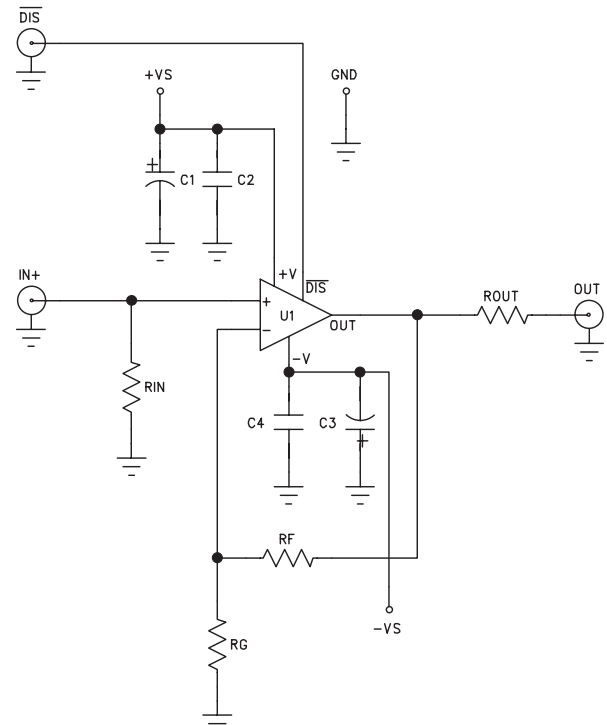
Figure 5: Evaluation Board Schematic
