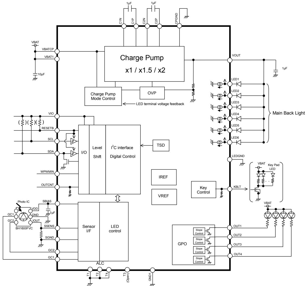
Fig.1 Block Diagram / Application Circuit example 1
