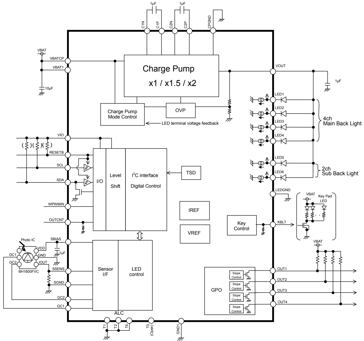
Fig.2 Block Diagram / Application Circuit example 2
