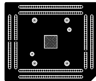
8 th layer(solder)
