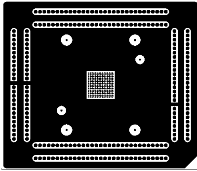
1 st layer(component)
