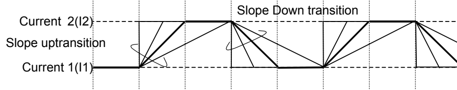
RGB wave setting timing diagram
