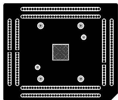
8 th layer (solder)
