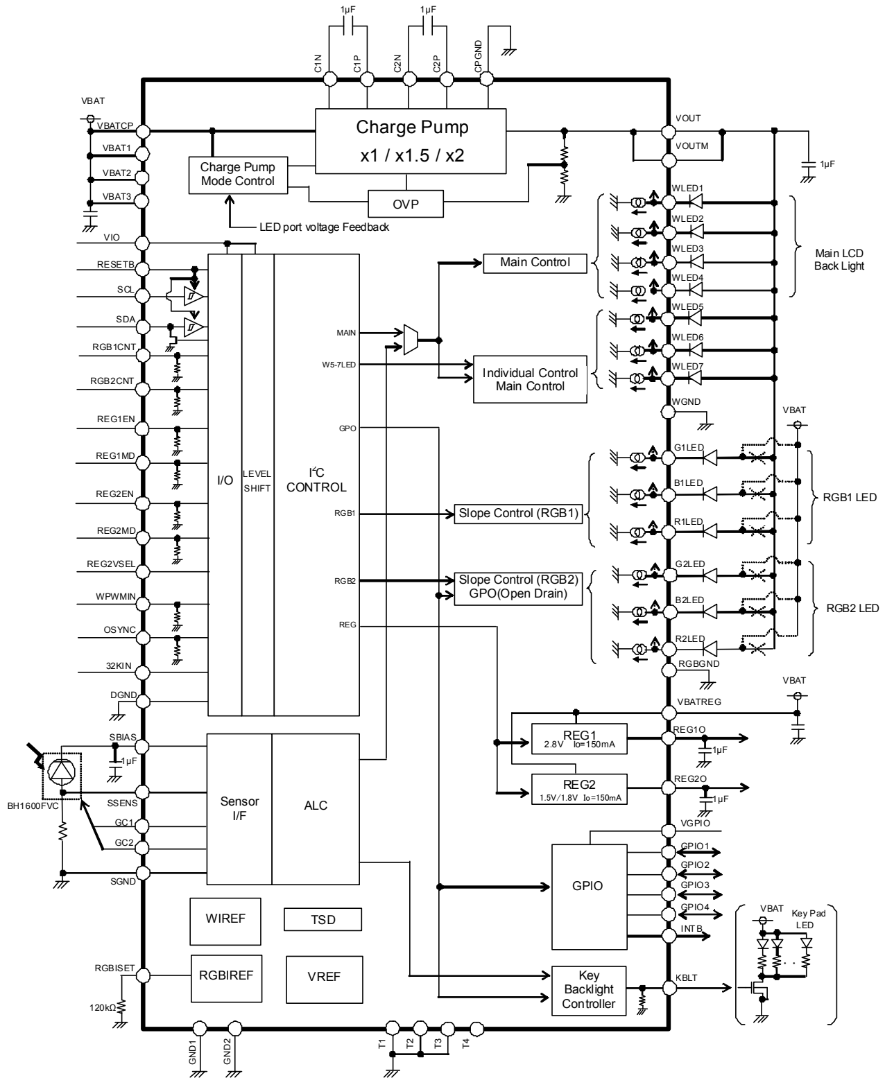
Block Diagram / Application Circuit example
