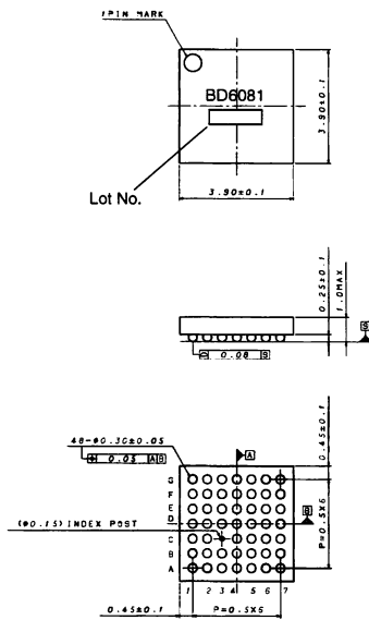
VCSP85H3 (48pins) (Unit : mm)
