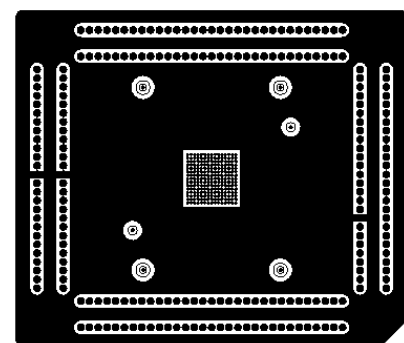
8 th layer(solder)
