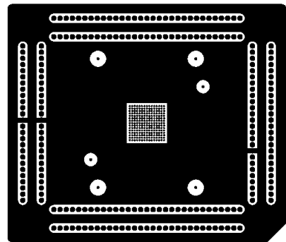
1 st layer(component)
