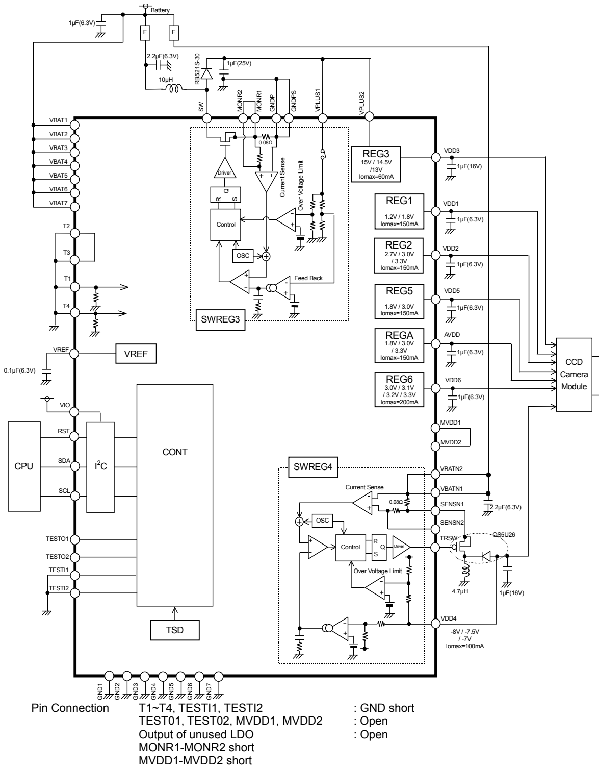
Fig.2 Block Diagram / Application Circuit example
