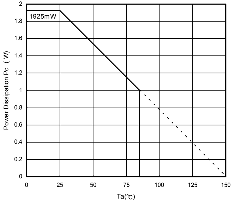
Fig.1 Power Dissipation
