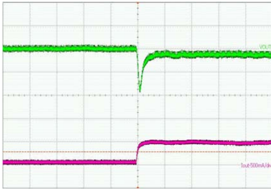
( V_{IN} = 5\text{ V} , I_{LOAD} = 100\text{ mA} , L = 3.3\ \mu\text{H} , C_{OUT} = 2 \times 22\ \mu\text{F} ) Upper Trace: Output Dynamic Voltage, 100 mV/div Lower Trace: Output Current, 500 mA/div
