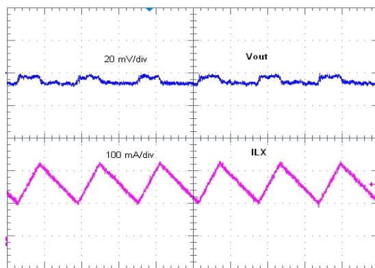
Figure 14. Step Down Converter PWM Mode Operation
