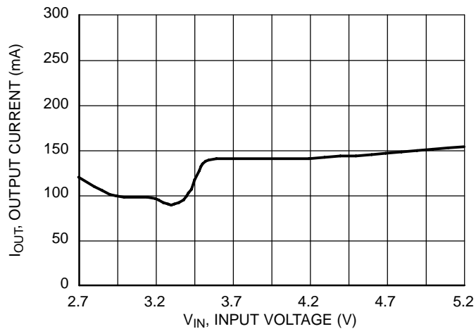
Figure 12. PFM/PWM Threshold vs. Input Voltage
