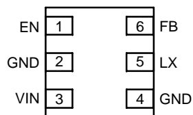
Figure 6. Pin Connections – UDFN6
